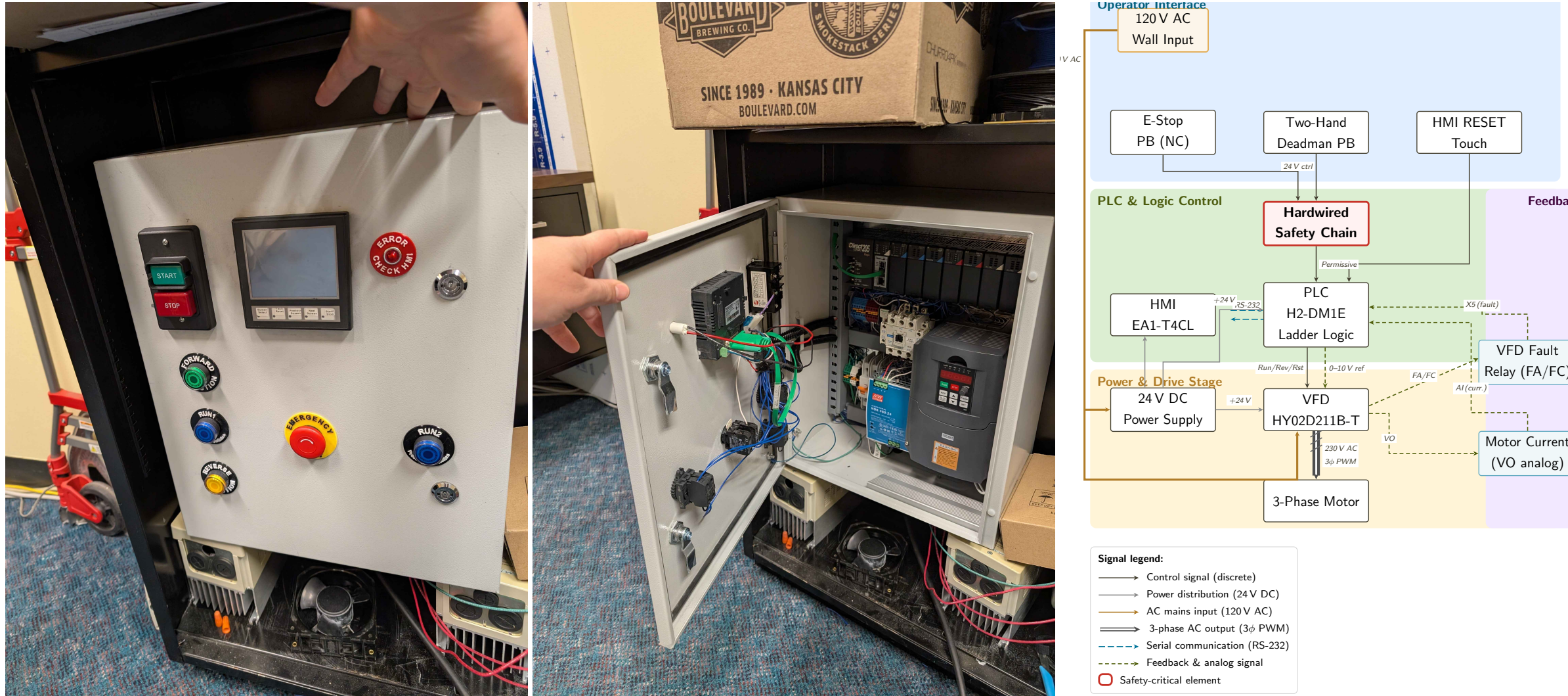
Operator face (left), panel interior (middle), and system block diagram (right): HMI, deadman / fwd / rev / E-stop, DirectLOGIC 205, Huanyang VFD, 24 V supply, SD-N35 contactor, terminal blocks; block diagram shows the signal path from AC in through the safety chain to the VFD and motor.
